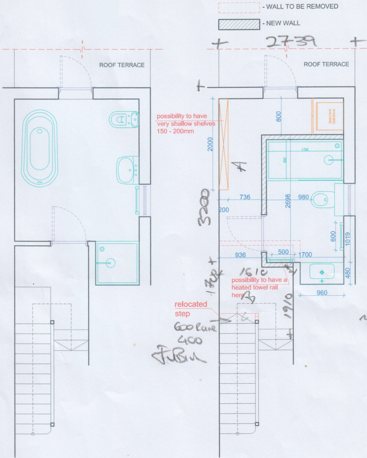
EXISTING BATHROOM PLAN
