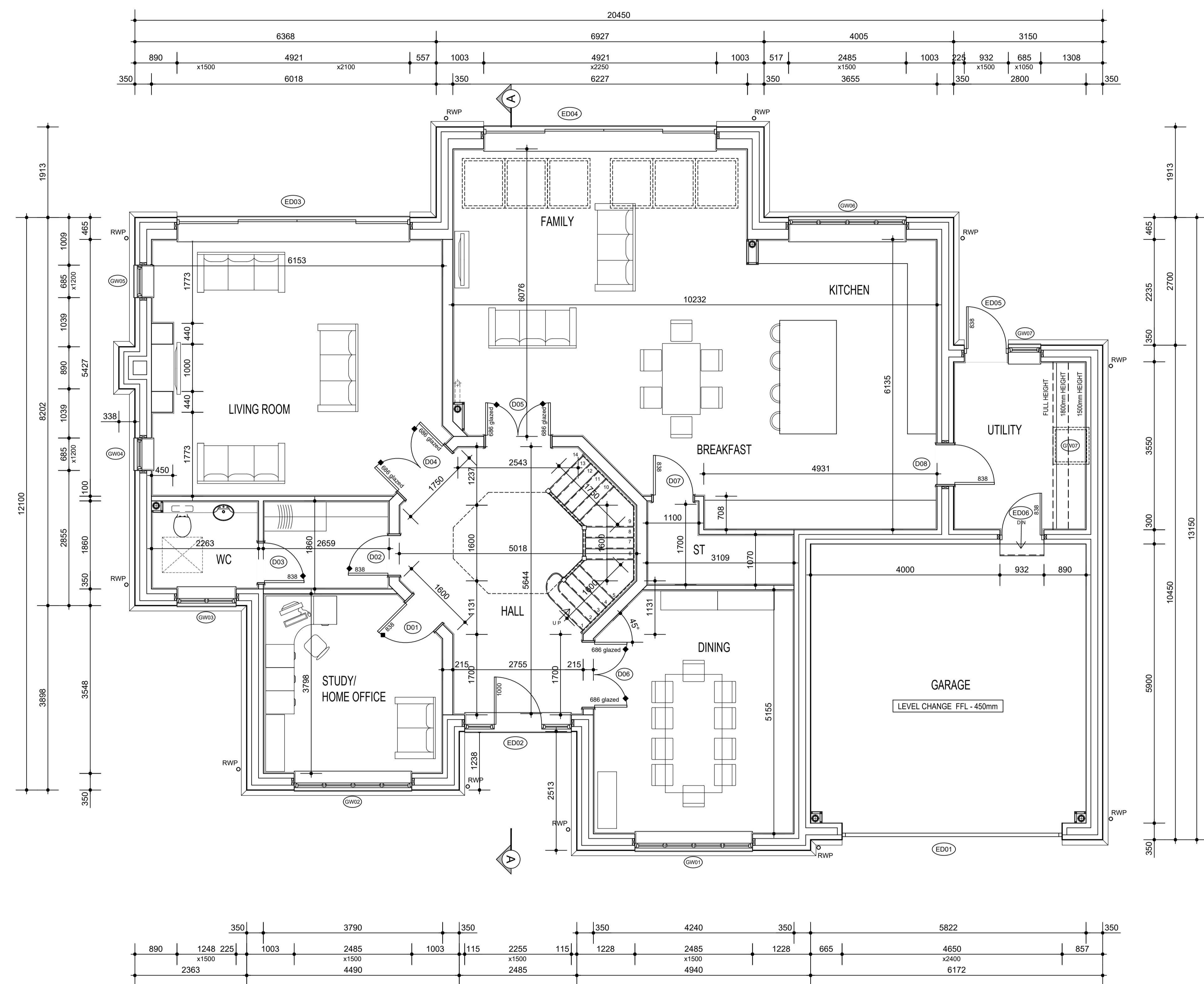
GROUND FLOOR LAYOUT - GA
