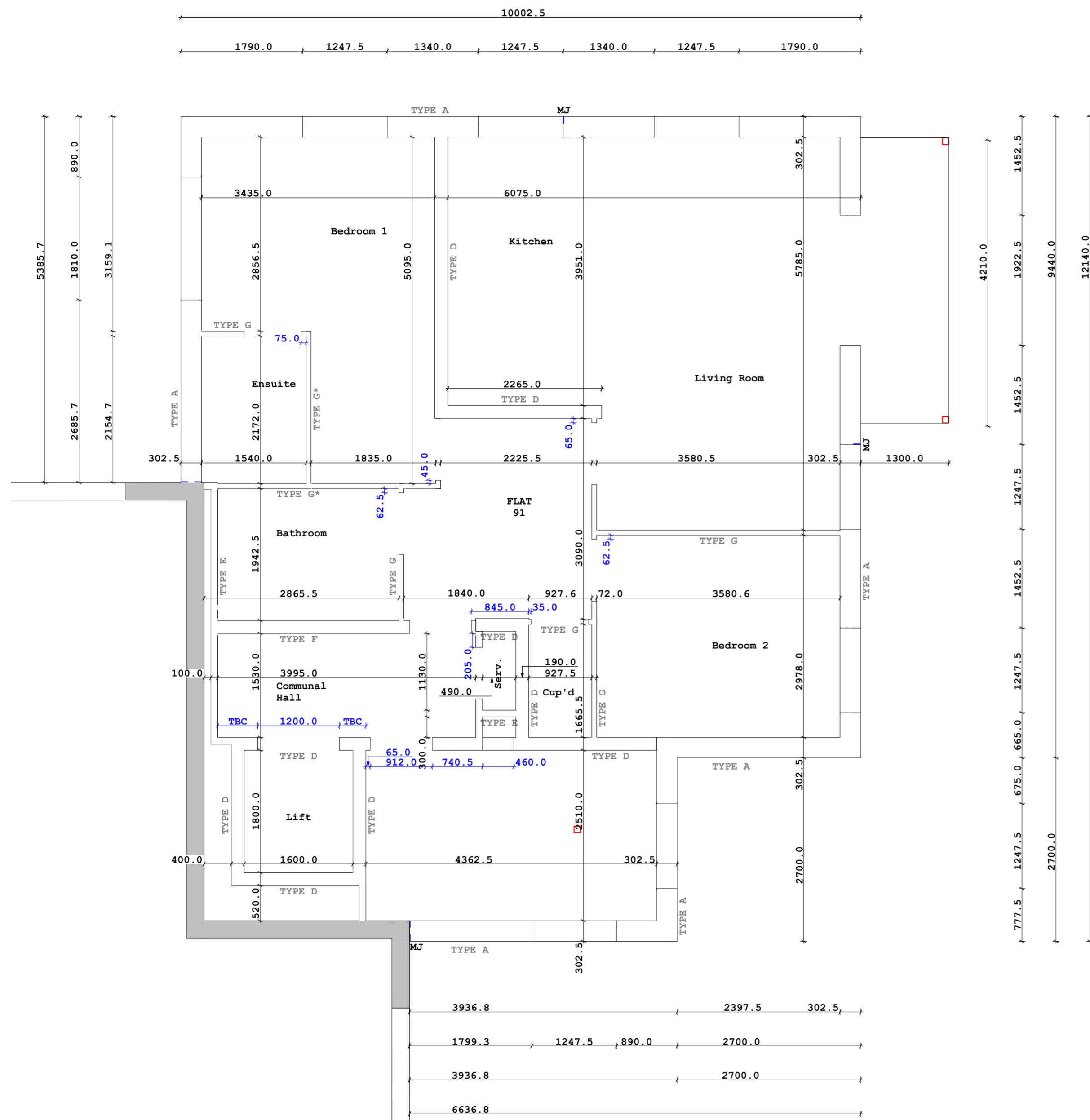
SECOND FLOOR SETTING OUT PLAN
