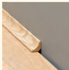
scotia 2400 X 19 X 19 MM 94.49 X 0.75 X 0.75 INCH
