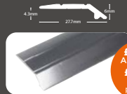
Vinyl Edge (Small) 4mm - M02
