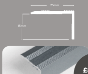
Nosings - 15mm Self-Adhesive - M75
