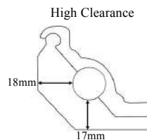
High Clearance
